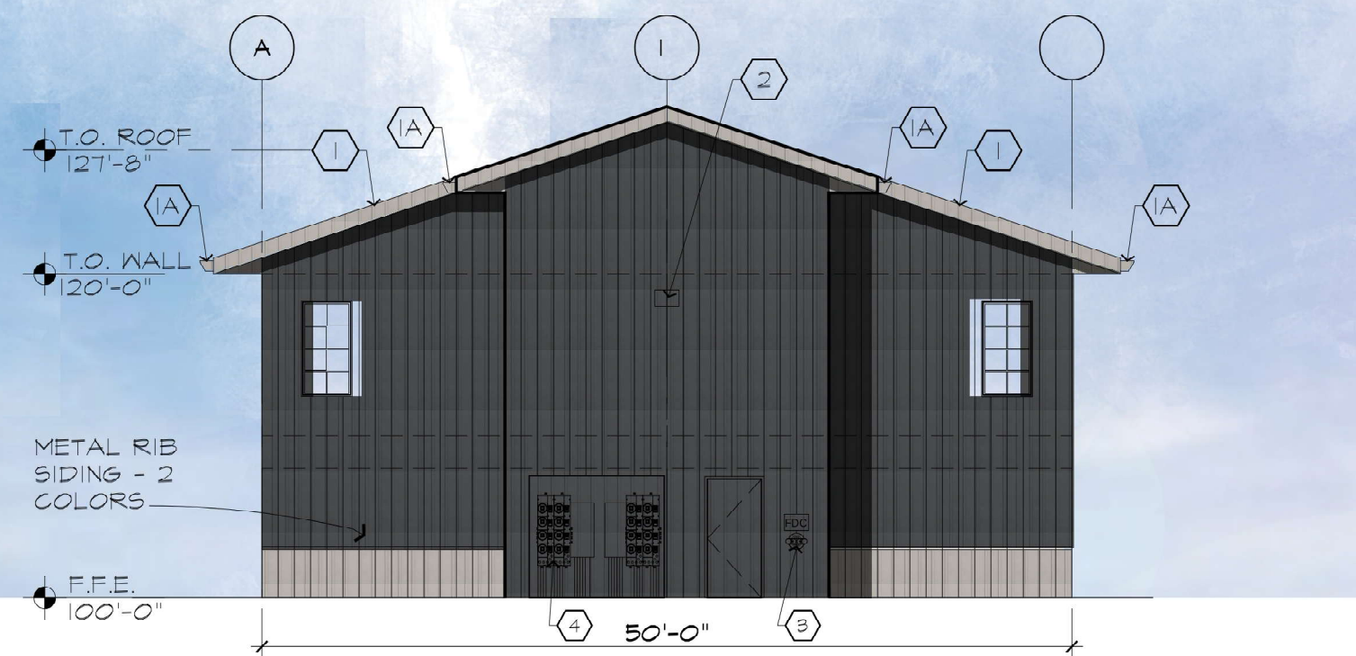
4 GARAGE CONDO - NORTH ELEV
