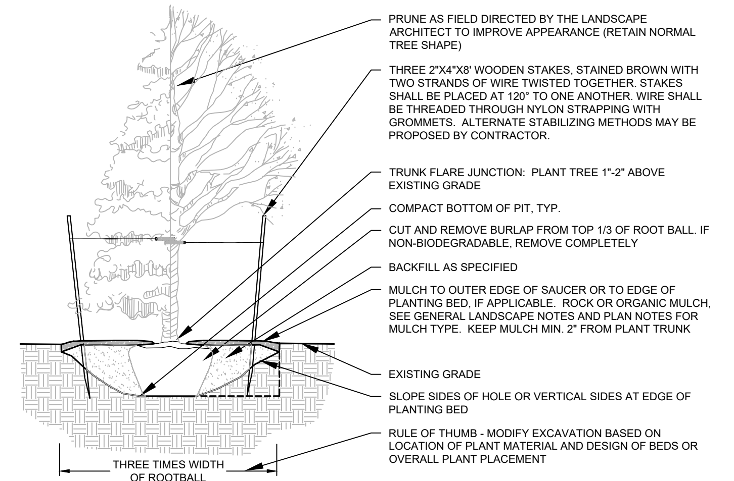
4 DECIDUOUS & CONIFEROUS TREE PLANTING N T S
