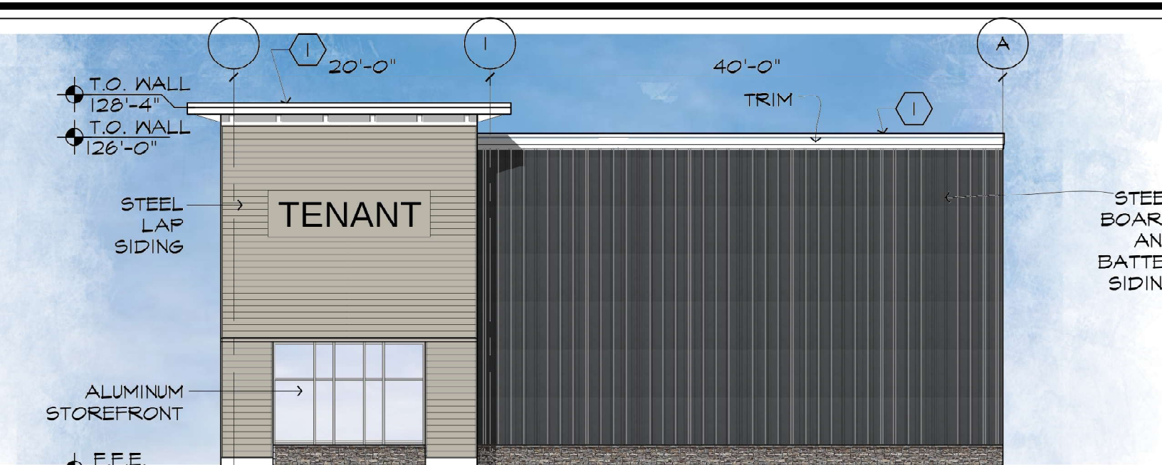
2 NORTH ELEVATION - OFFICE/WAREHOUSE 3/32" = 1'-0"
